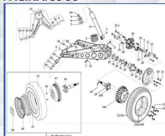
LAMINA-24 SUSPENSION TRASERA (TAMBOR, COPLE, BALEROS, AMORTIGUADOR) PAGINA: 55-58
